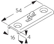
SG 6124 Bracket
