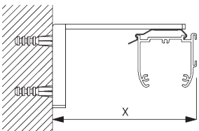
Smart Fix SG 11200 - SG 11205 and bracket SG 2616: Screw SG 10395 (M4x6) needed.
