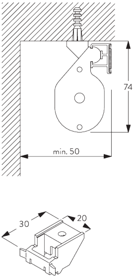
SG 3603 Bracket
