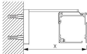
Smart Fix SG 11200 - SG 11204 and bracket SG 2521: Screw SG 10395 (M4x6) needed.
