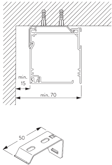
SG 2521 Bracket
