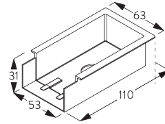
SG 11886 Recess mask
