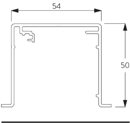
SG 11865 Recess profile
