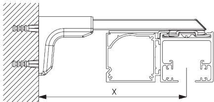
Universal Smart Fix SG 11155 - SG 11156 and clamp SG 3044: Screw SG 11158 (M4x12) needed.
